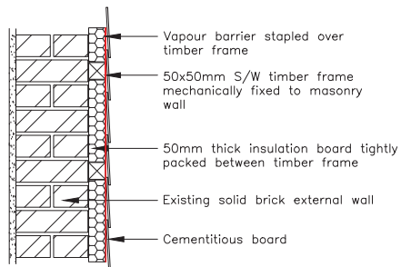
External wall finish Detail Not to scale
